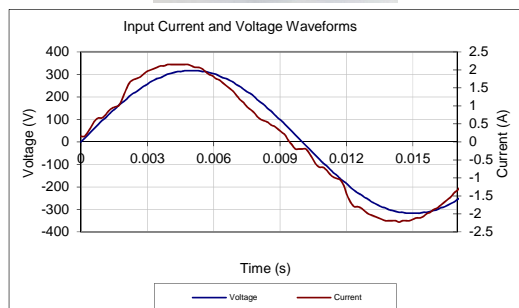
Input AC Current Waveform (ITHD = 9.7%, 50% Load)
