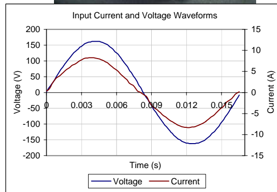
Input AC Current Waveform (ITHD = 6.95%, 50% Load)
