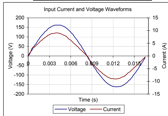
Input AC Current Waveform (ITHD = 7.32%, 50% Load)
