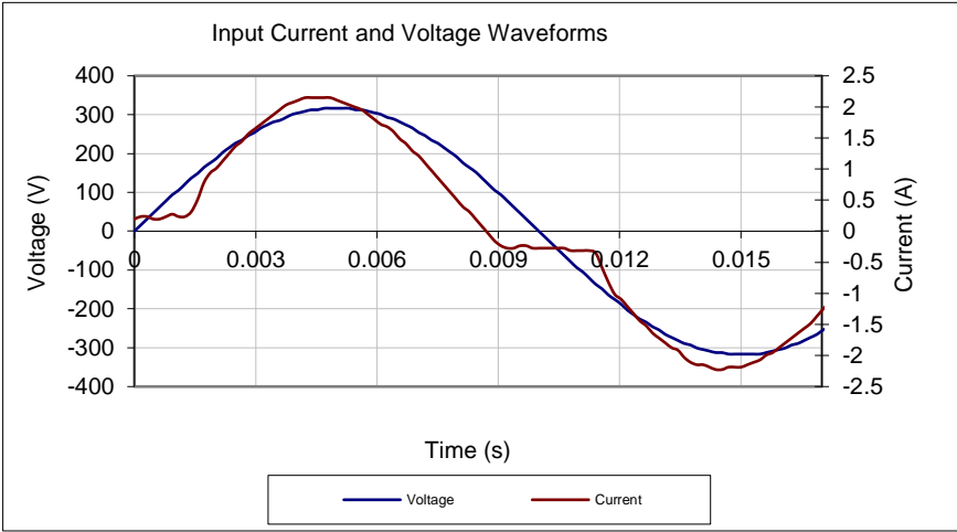
Input AC Current Waveform (ITHD = 23.54%, 50% Load)
