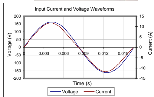
Input AC Current Waveform (THD = 6.04%, 50% Load)
