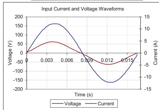
Input AC Current Waveform (ITHD = 4.81%, 50% Load)
